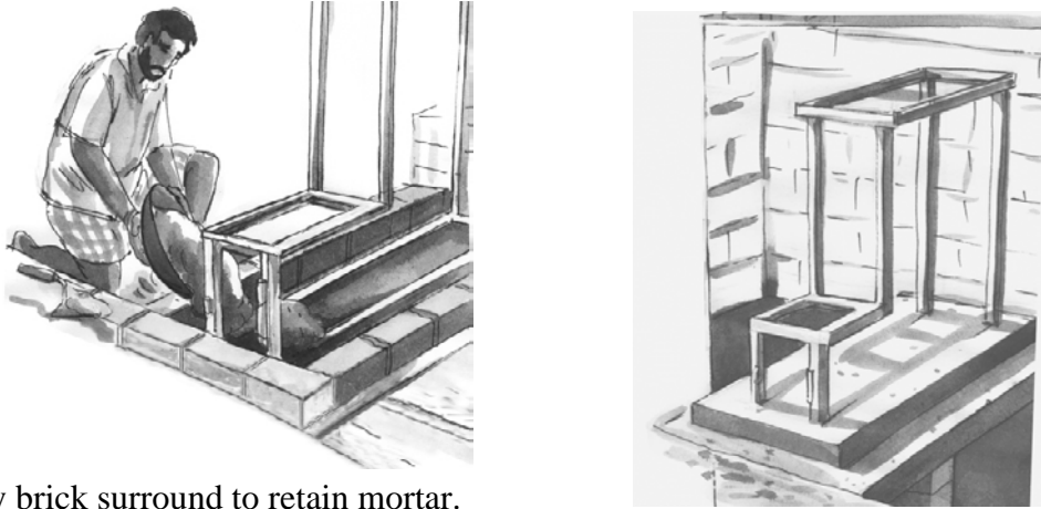
Figure 2.3.5 Placing metallic frame and grouting frame in PCC slab
